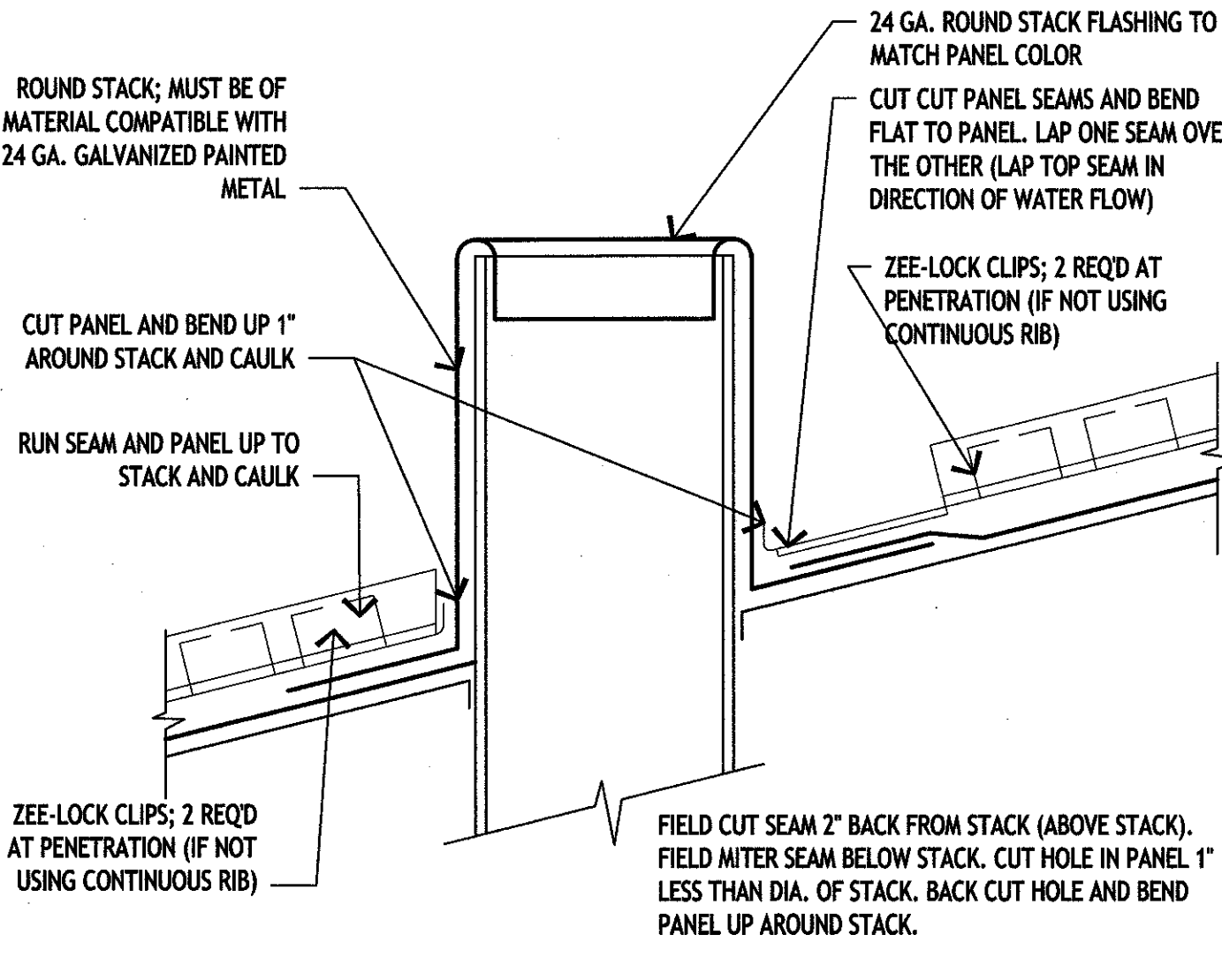
E-9 ROOF PENETRATION DETAIL 3"-1'-0" @ STANDING SEAM
