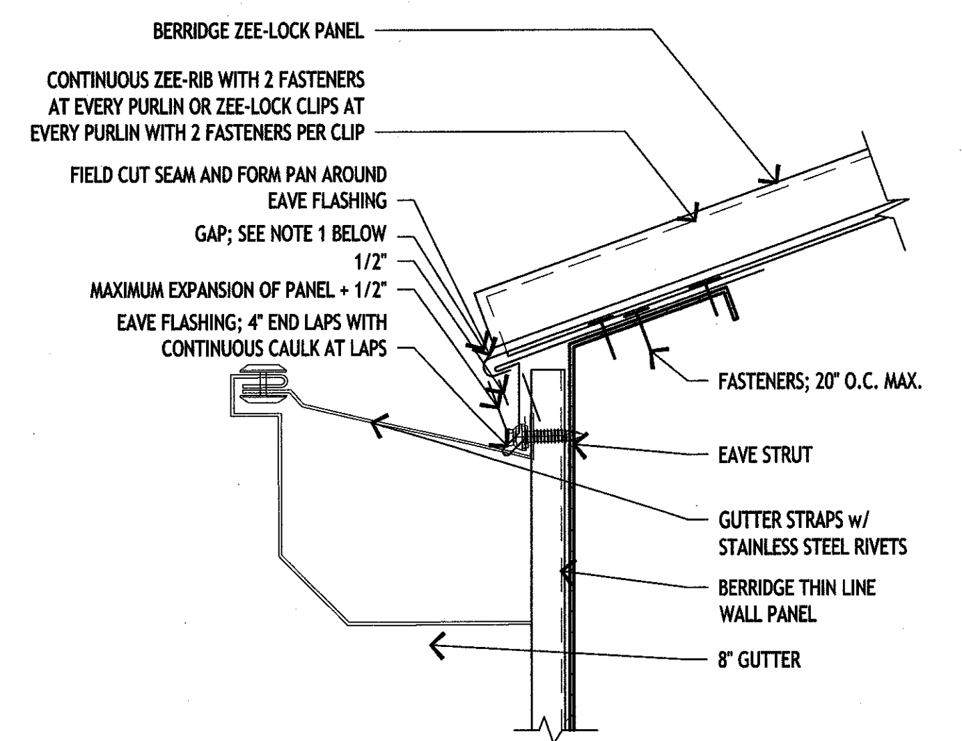
A-13 EAVE DETAIL 3"-1'-0"
