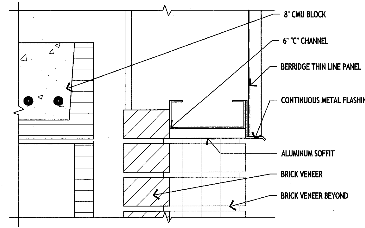
J-9 SOFFIT DETAIL 3"-1'-0"
