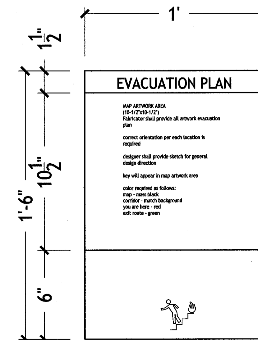
A-13 EVACUATION ROUTE - TYPE 7
