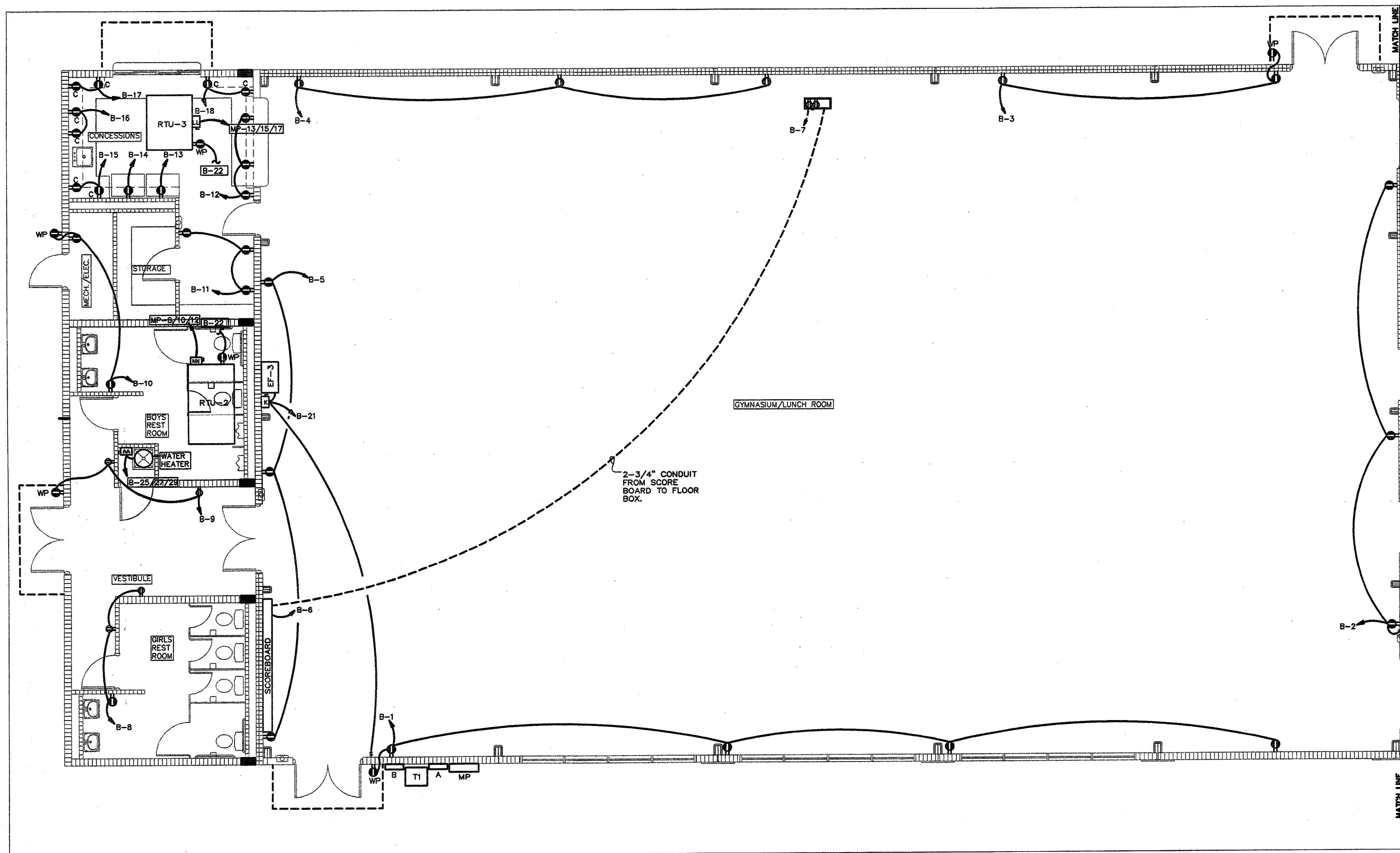
1 ELECTRICAL POWER PLAN SCALE: 3/16" = 1'-0"
