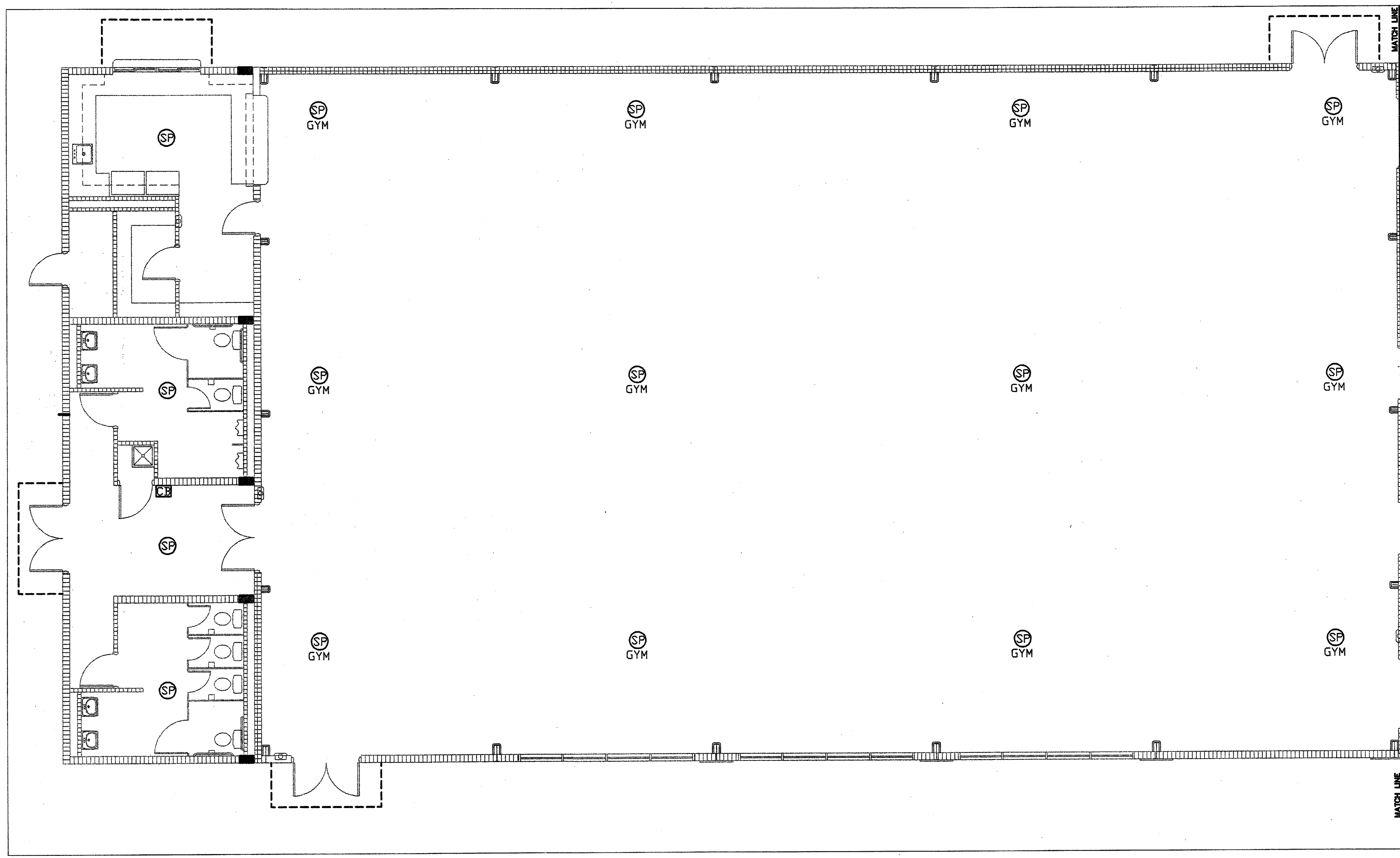
1 INTERCOM PLAN E5 SCALE: 3/16" = 1'-0"
