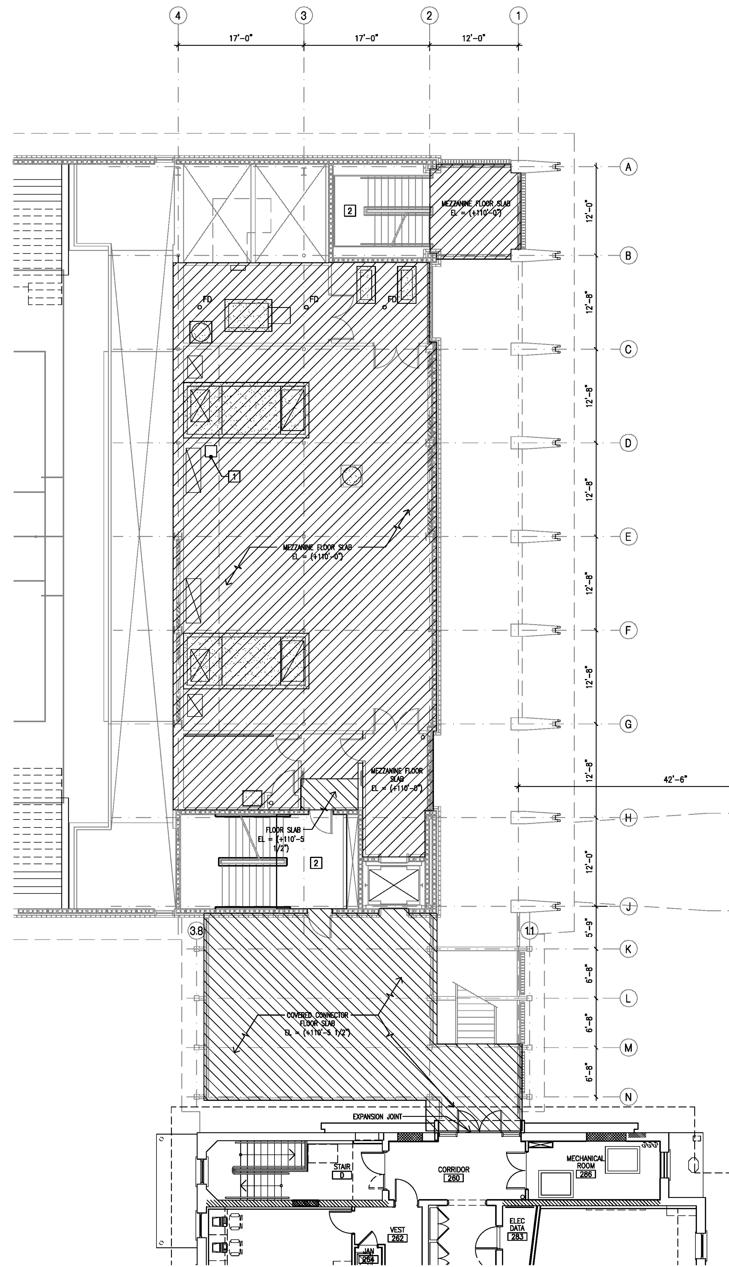
1 MEZZANINE FLOOR SLAB PLAN A201M Scale: 1/8" = 1'-0"
