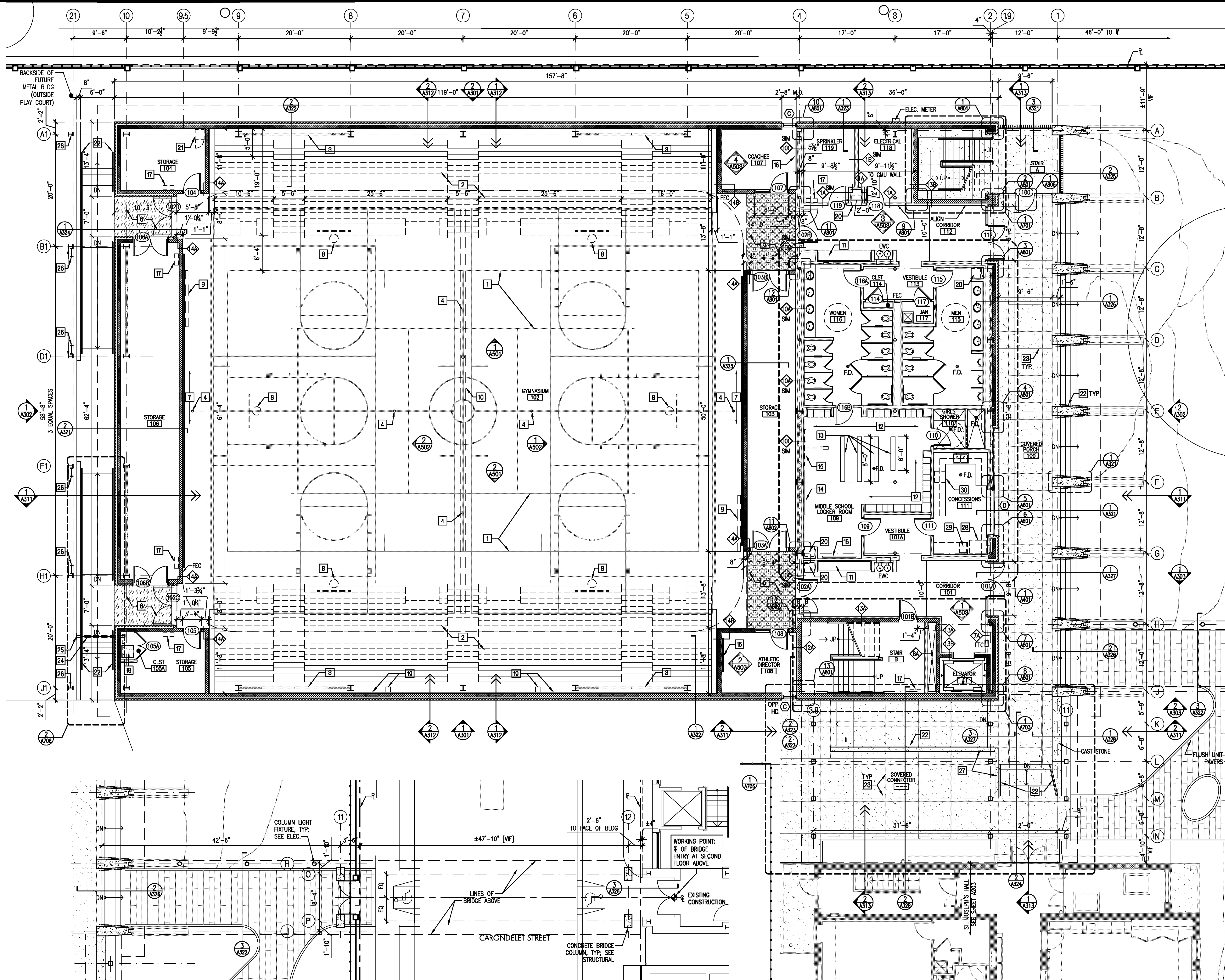
2 FIRST FLOOR PLAN - NEW BRIDGE SUPPORTS Scale: 1/8" = 1'-0"
