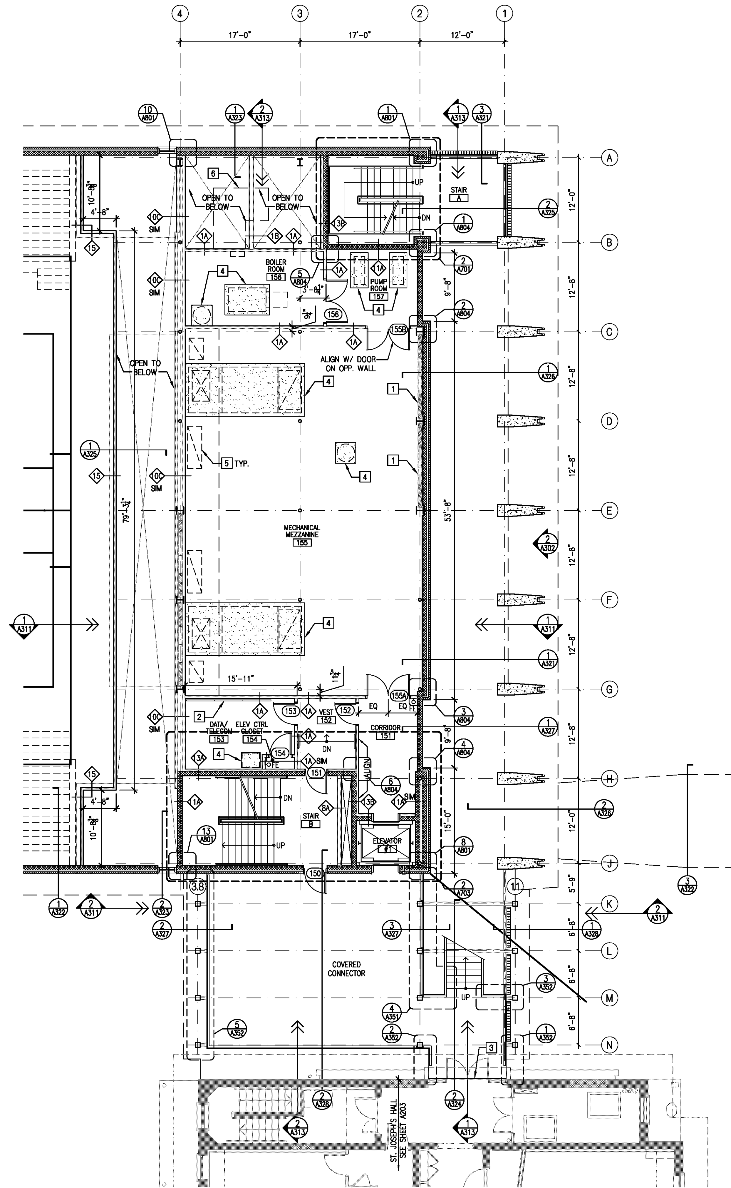
1 MECHANICAL MEZZANINE PLAN - NEW BUILDING A201M Scale: 1/8" = 1'-0"
