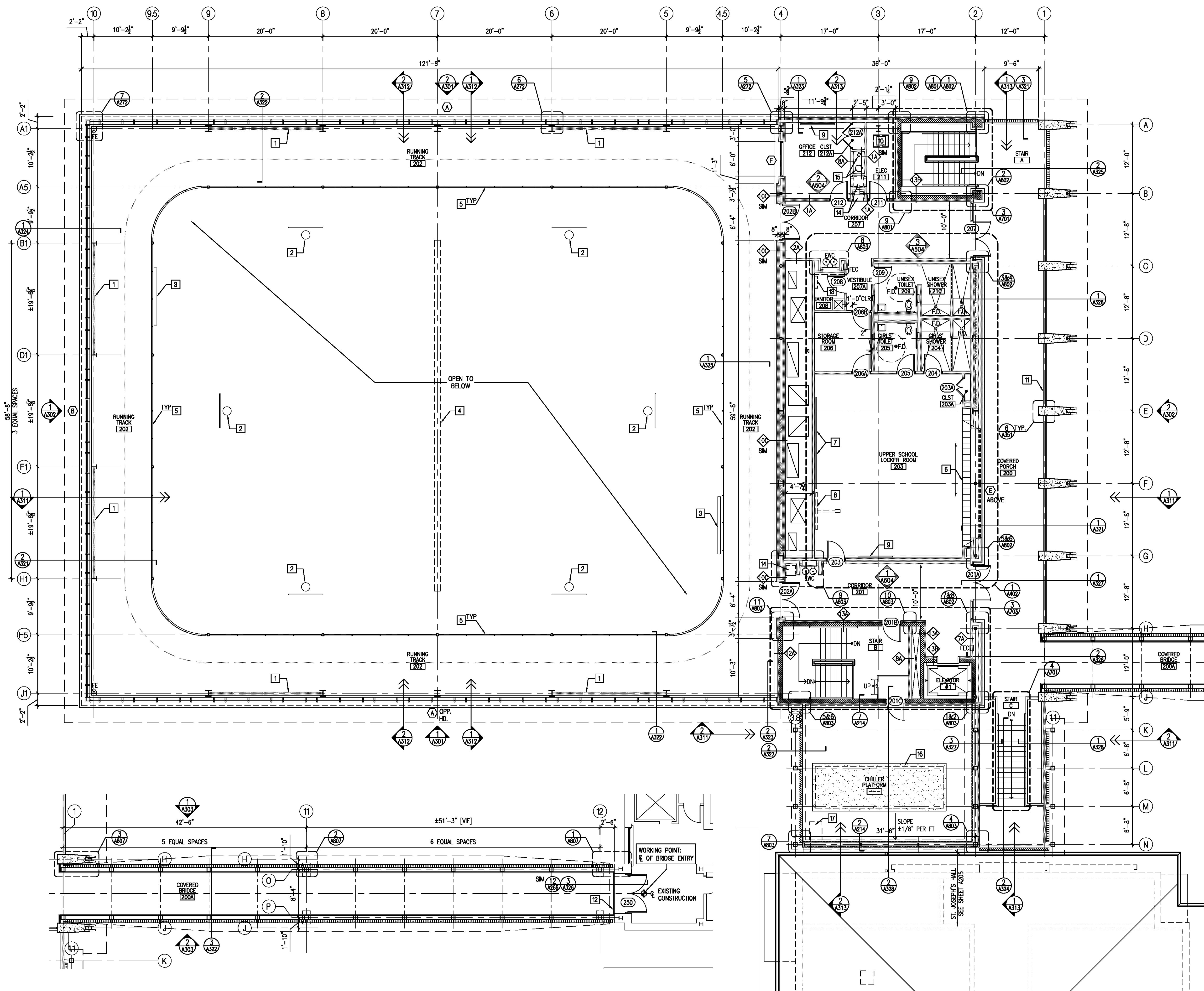
2 SECOND FLOOR PLAN - NEW BRIDGE A202 Scale: 1/8" = 1'-0"
