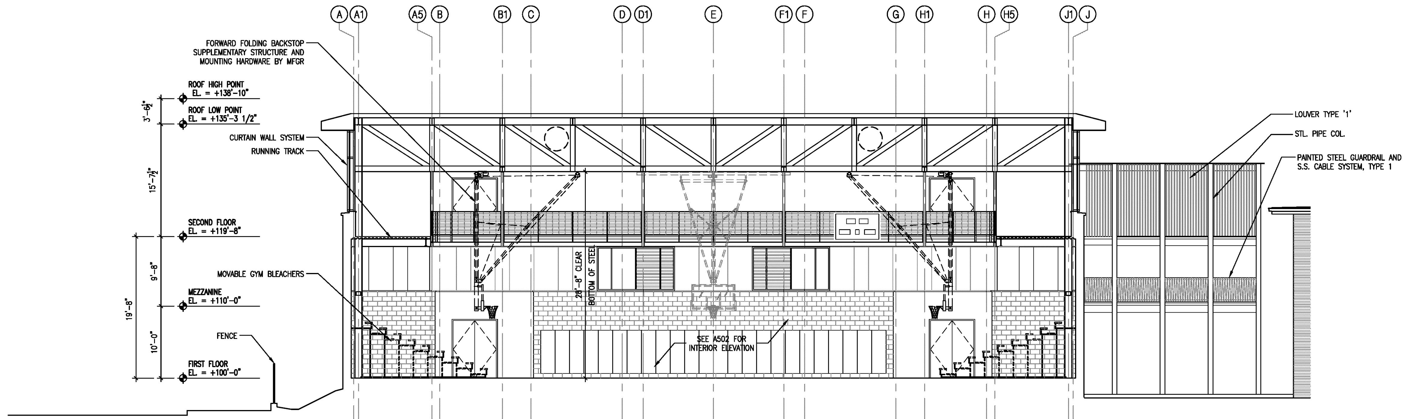
1 SECTION THROUGH GYM A201 | A312 LOOKING SOUTH Scale: 1/8"=1'-0"
