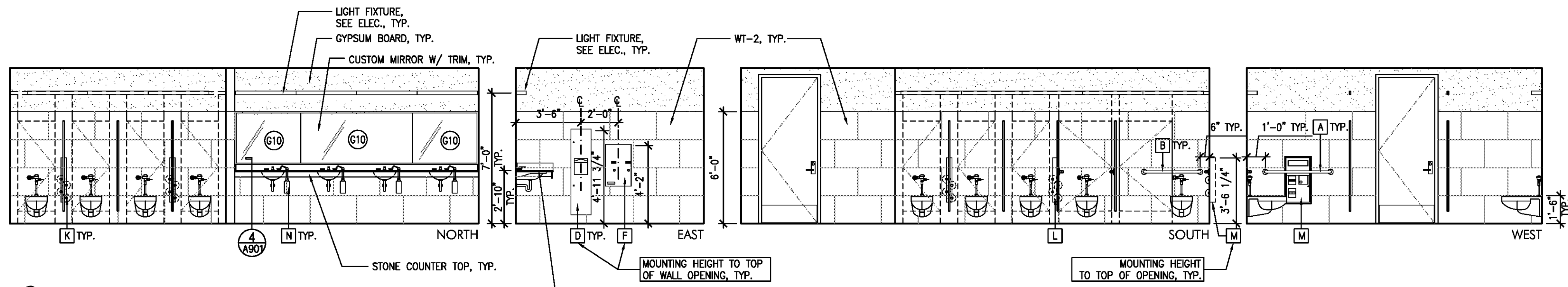
2 A401 INTERIOR ELEVATIONS WOMEN 116 Scale: 1/4" = 1'-0"
