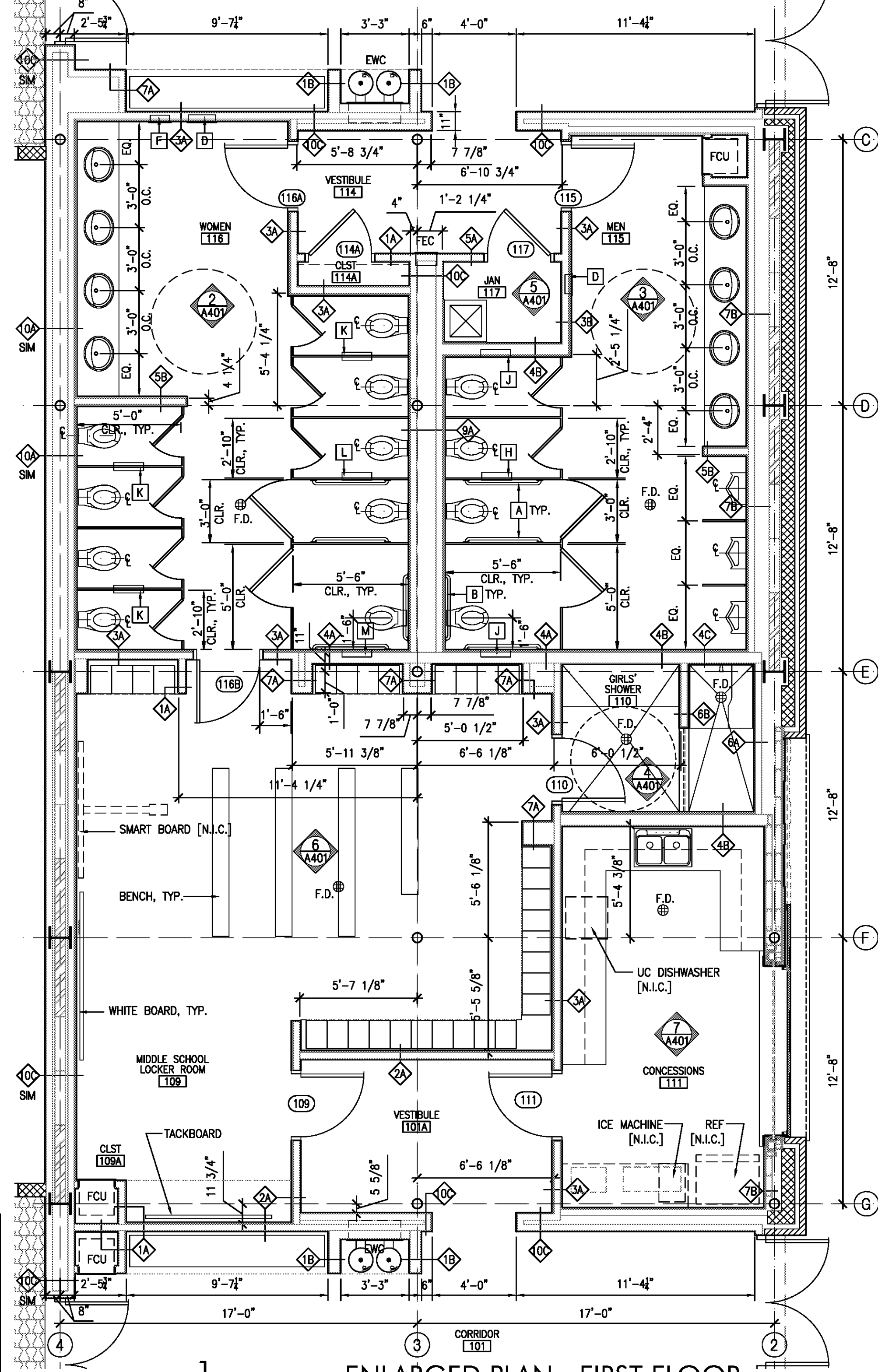
1 A201 A401 ENLARGED PLAN - FIRST FLOOR TOILETS, LOCKERS, CONCESSIONS Scale: 1/4" = 1'-0"
