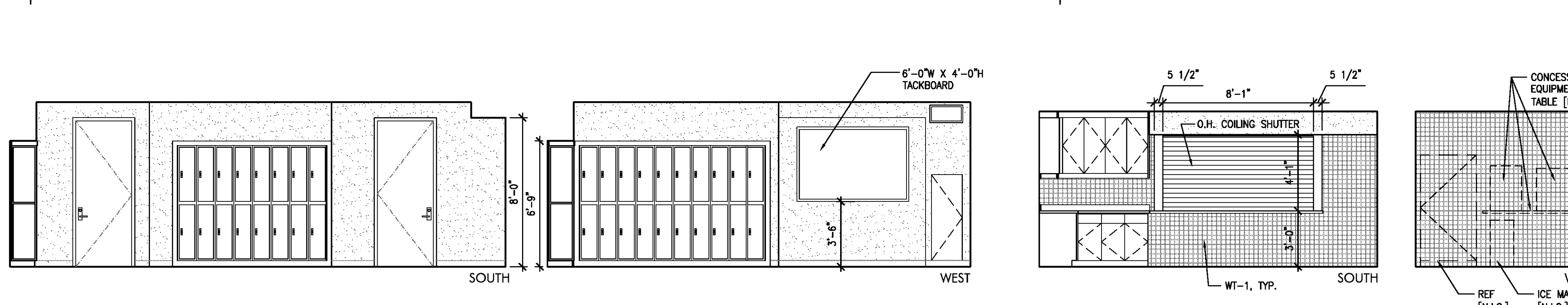
6 A401 INTERIOR ELEVATIONS LOCKER ROOM 109 Scale: 1/4" = 1'-0"
