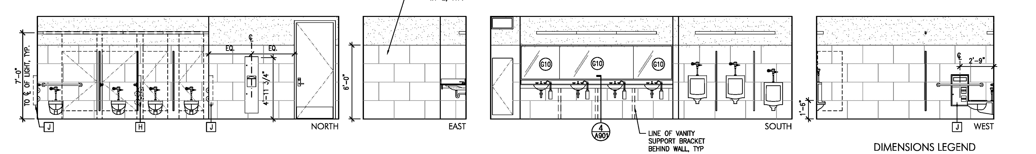
3 A401 INTERIOR ELEVATIONS MEN 115 Scale: 1/4" = 1'-0"
