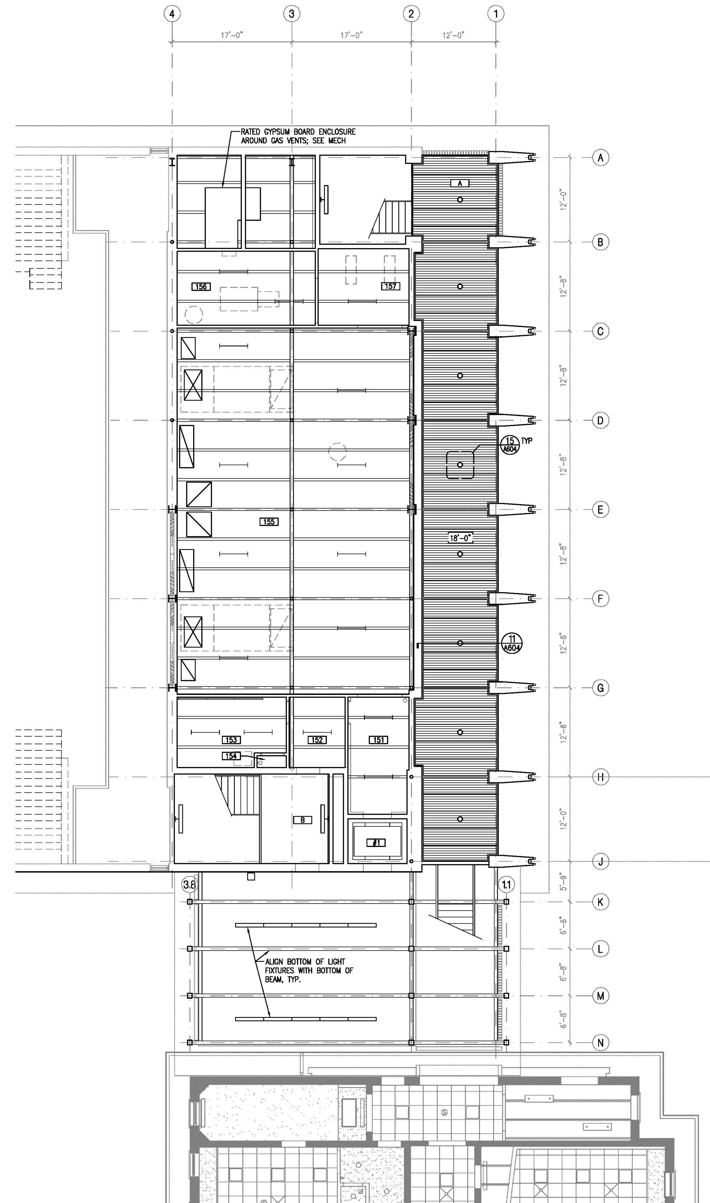
1 MECHANICAL MEZZANINE RCP - NEW BUILDING A601M Scale: 1/8" = 1'-0"
