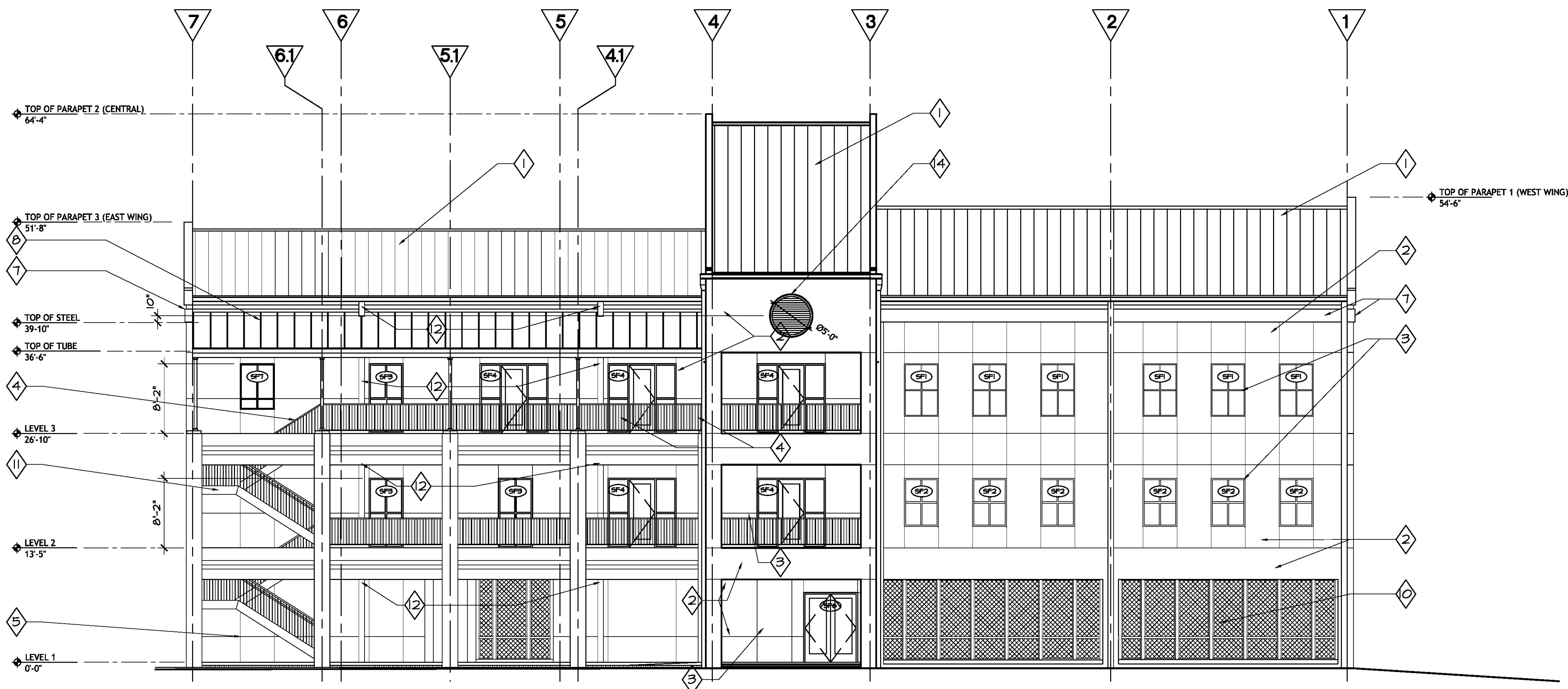
1. BUILDING ELEVATION - NORTH SCALE: 1/8" = 1'-0"
