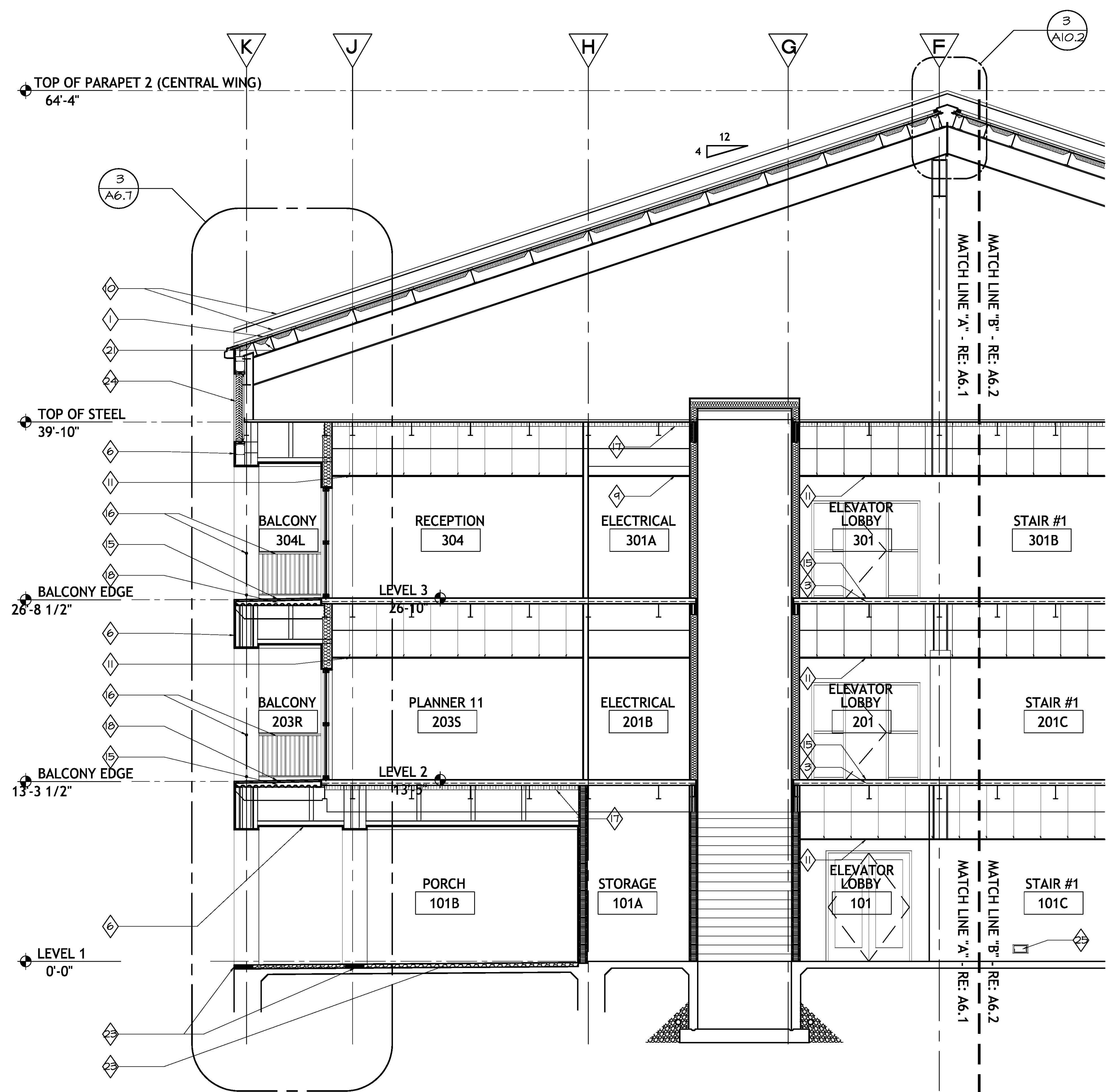
1. BUILDING SECTION - CROSS "A" SCALE: 1/4" = 1'-0"
