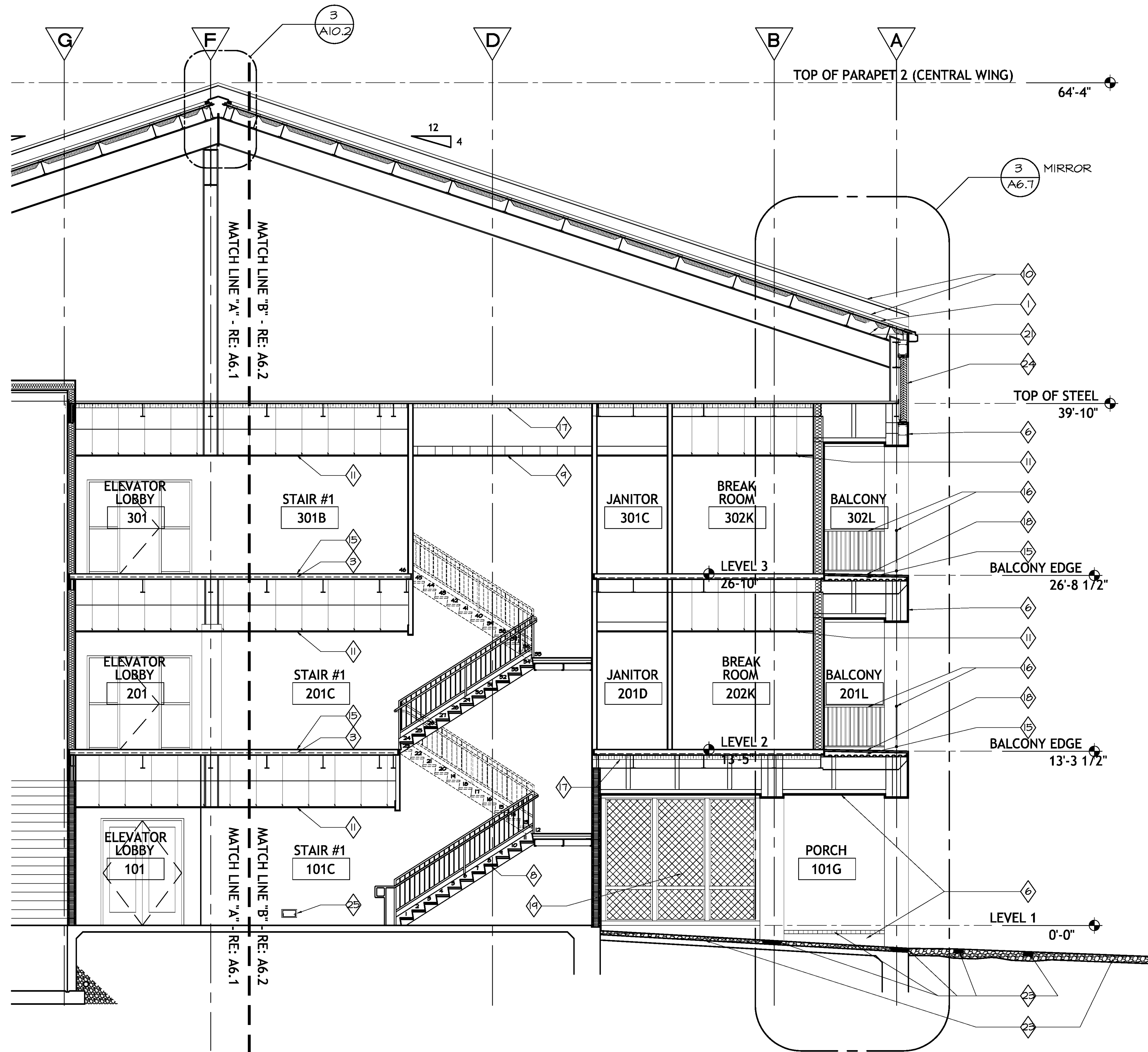
1. BUILDING SECTION - CROSS "B" SCALE: 1/4" = 1'-0"
