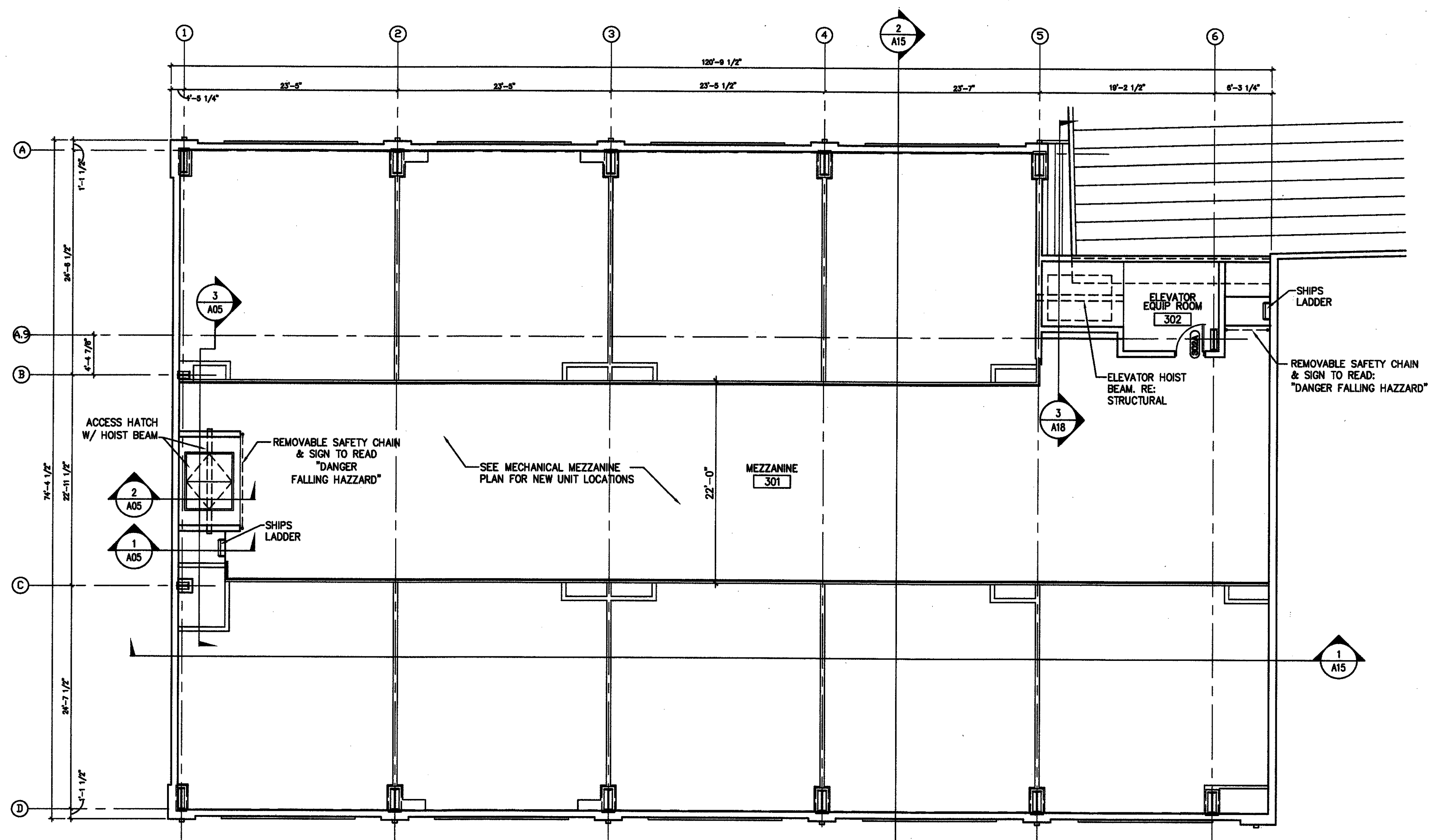
2 EXISTING MEZZANINE PLAN A04 1/8" = 1'-0" PHASE 2
