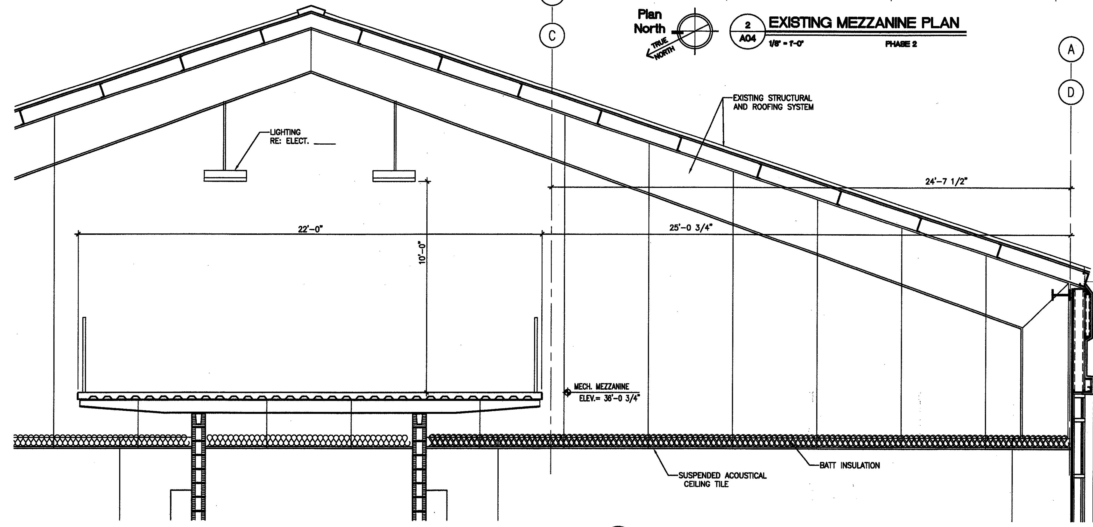
1 EXISTING MEZZANINE SECTION A04 3/8" = 1'-0" PHASE 2
