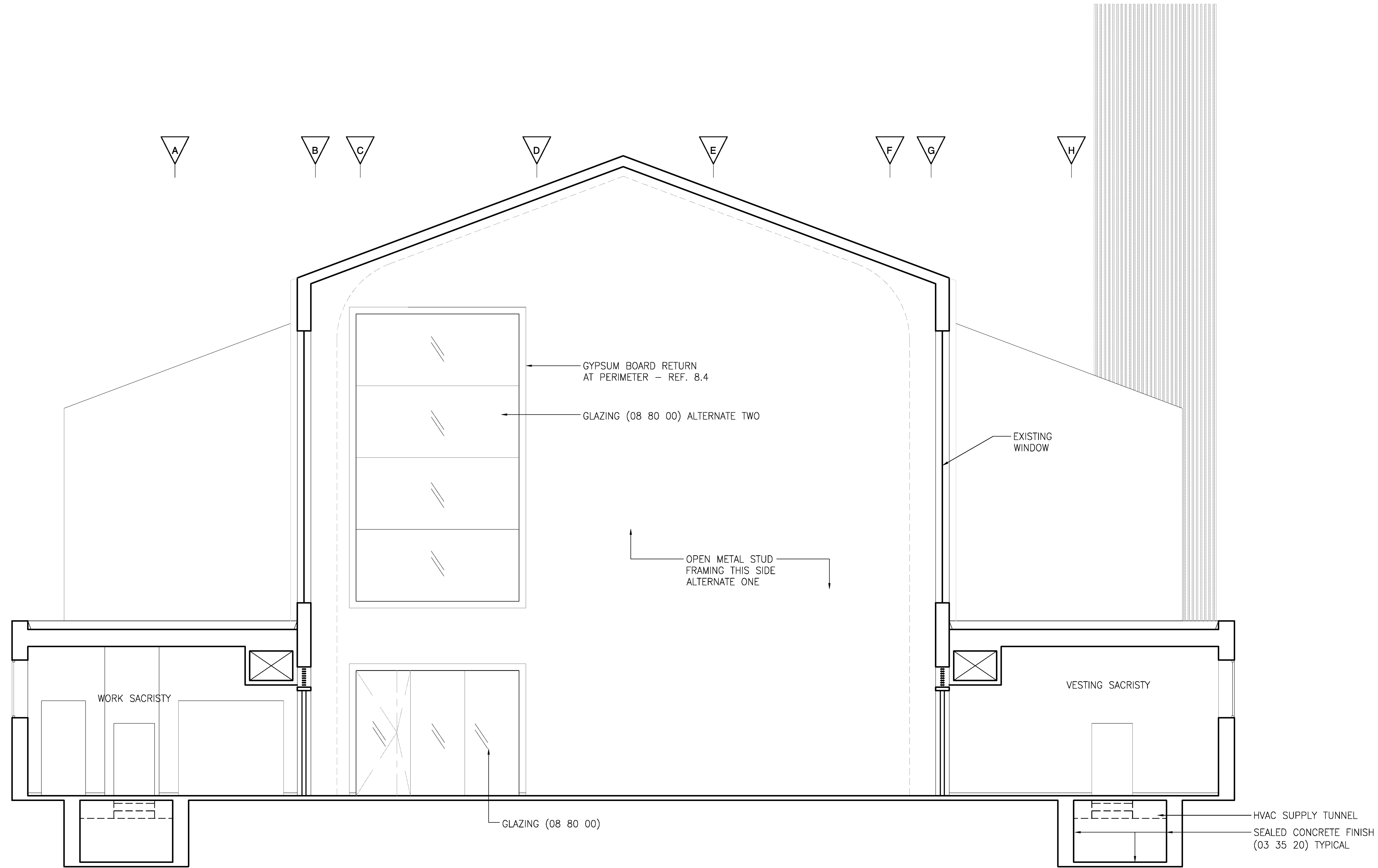
SECTION THRU CHAPEL 2.1 | 5.6 TOWARD SANCTUARY 1/4" = 1'-0"
