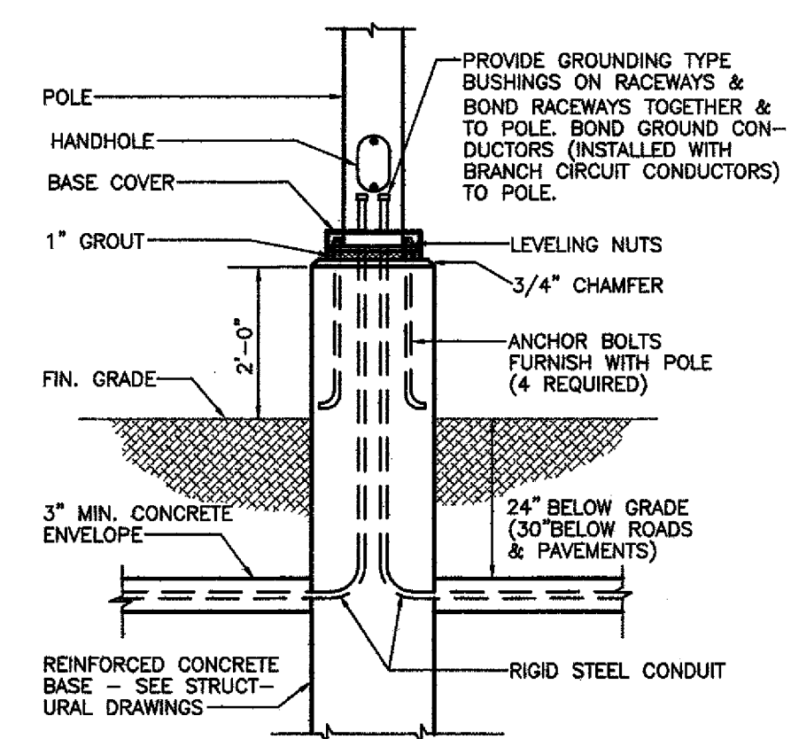
ELECTRICAL POLE BASE DETAIL NOT TO SCALE NOTE: 1. SOME LOCATIONS MAY REQUIRE ONE AND/OR SEVERAL CONDUITS.
