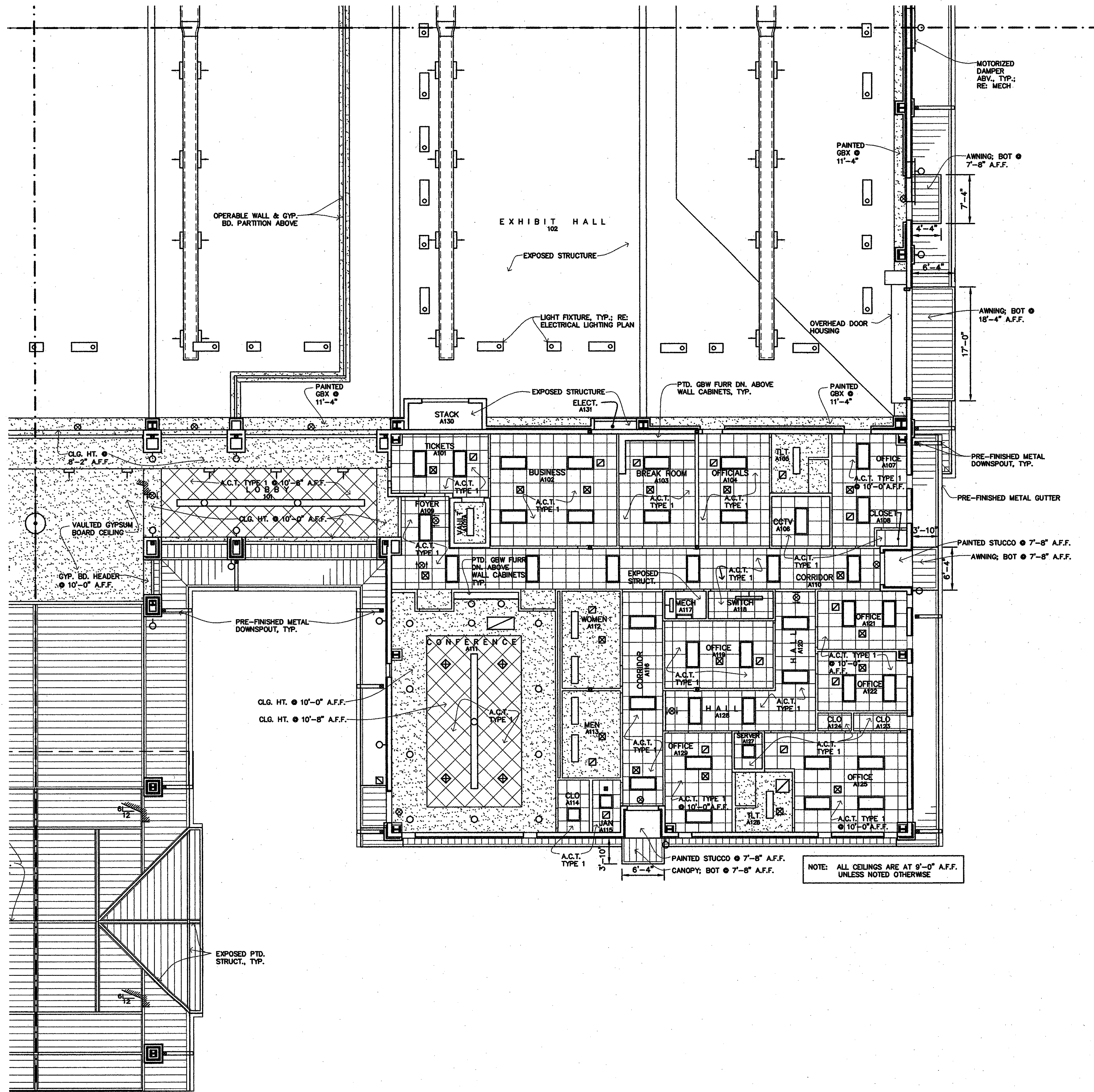
1 AREA 'A' CEILING PLAN A2.6 | A2.6 1/8" = 1'-0"
