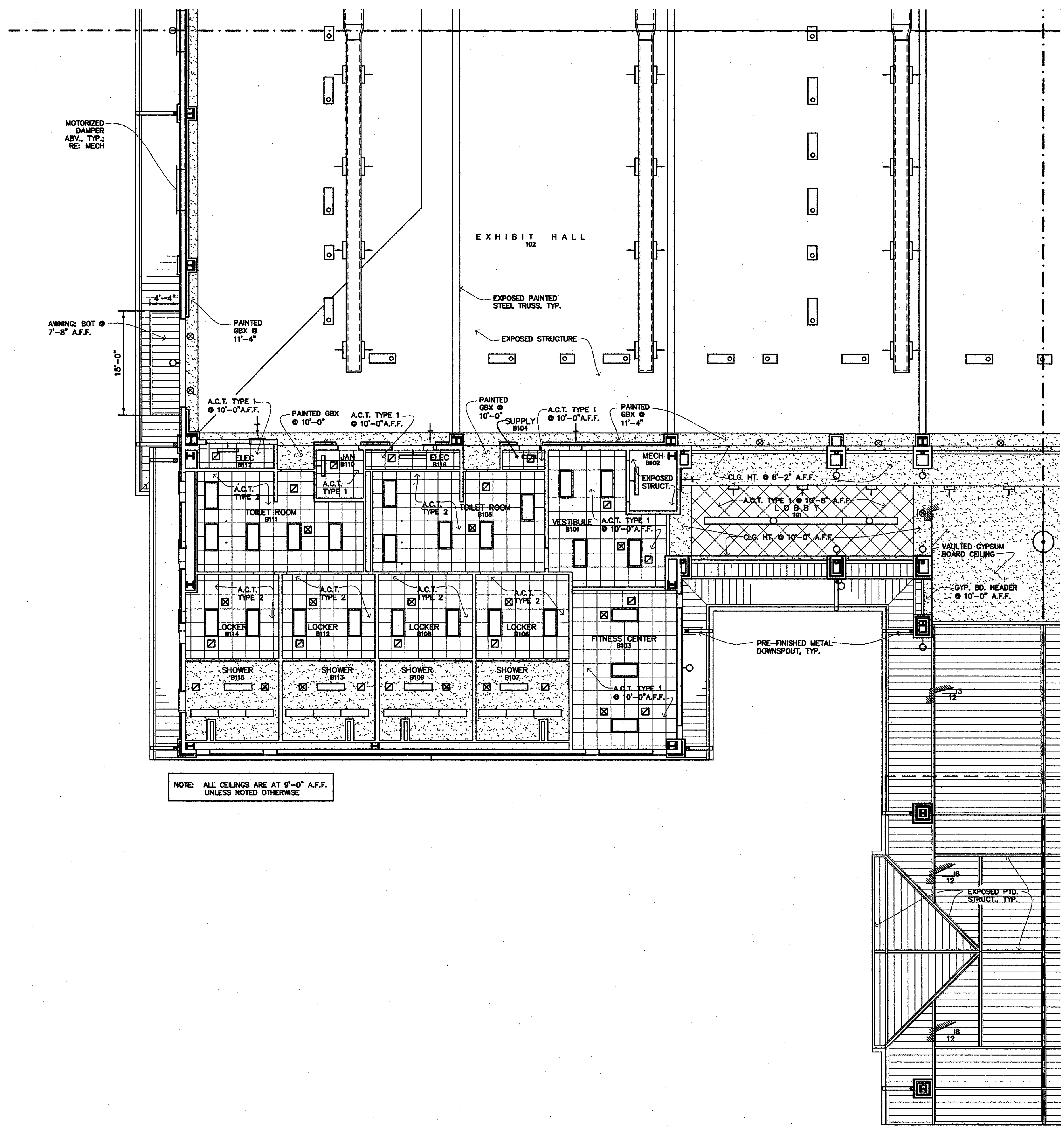
1 AREA 'B' CEILING PLAN A2.7 | A2.7 1/8" = 1'-0"
