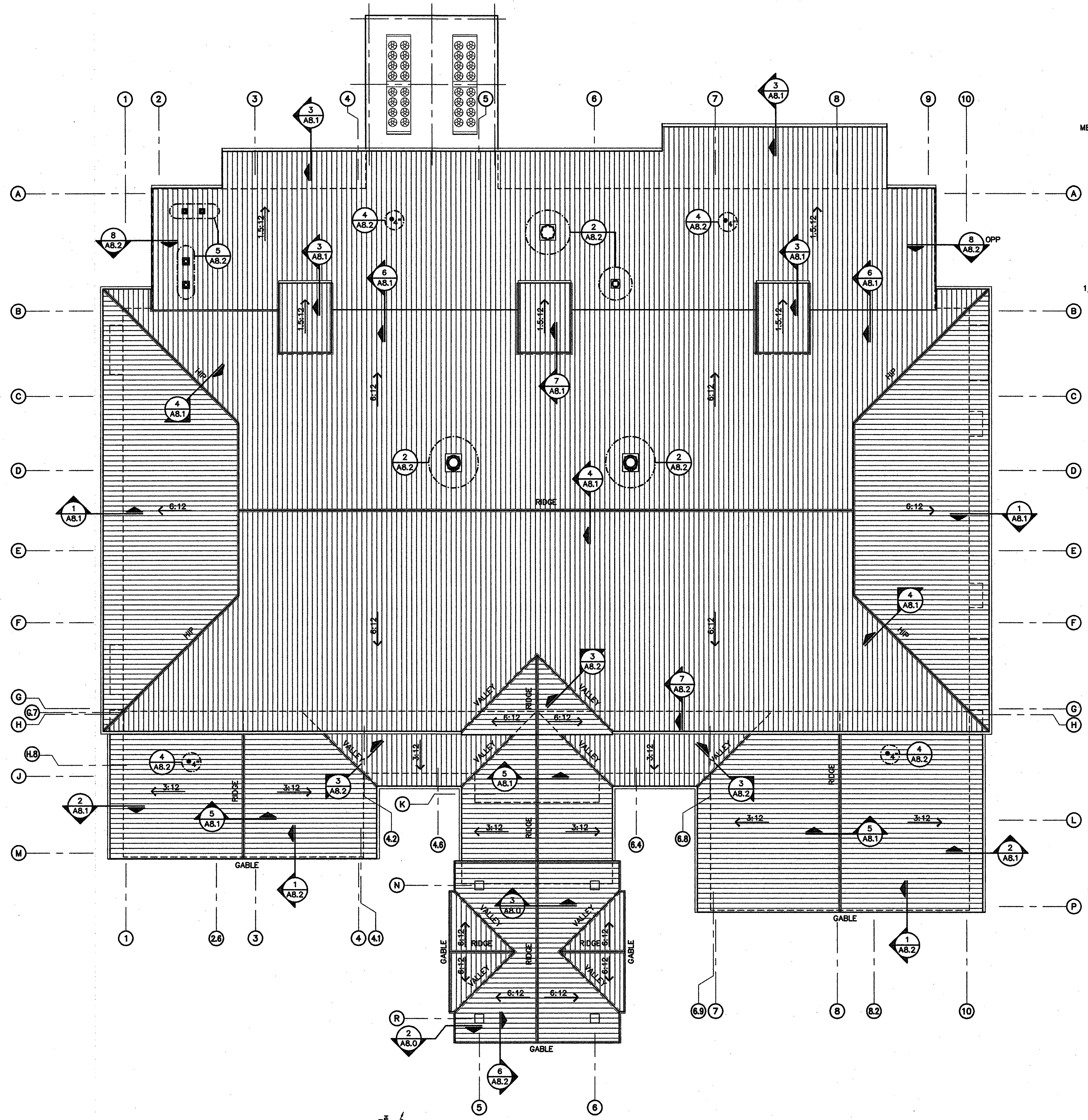
1 BUILDING ROOF PLAN A8.0 | A8.0 1/16" = 1'-0"
